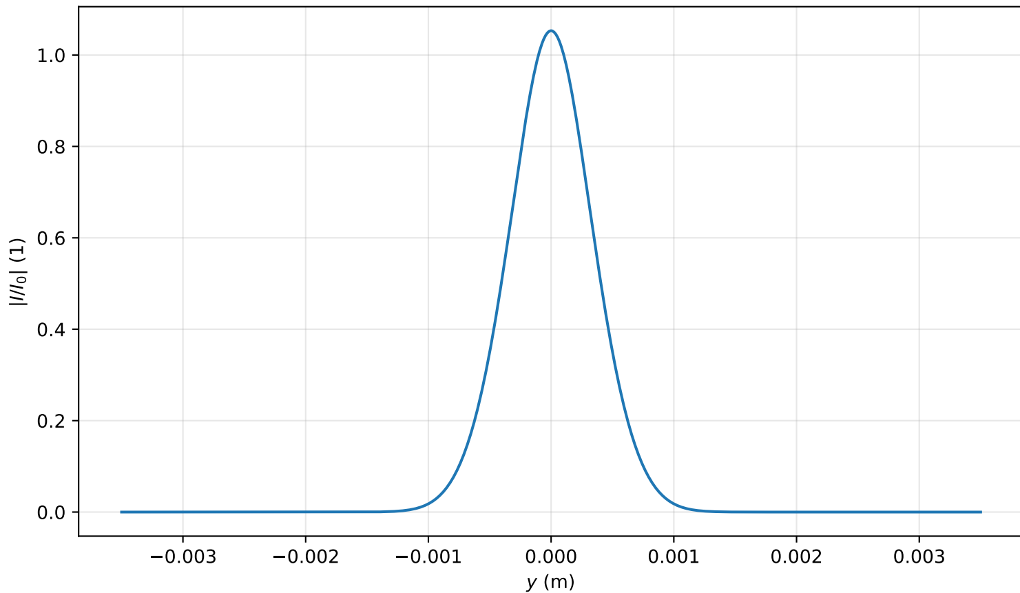
Intensity profile I(x=0, y, z=0.318)/I_0 , P_{in}=0.8P_{cr} , artificial time
